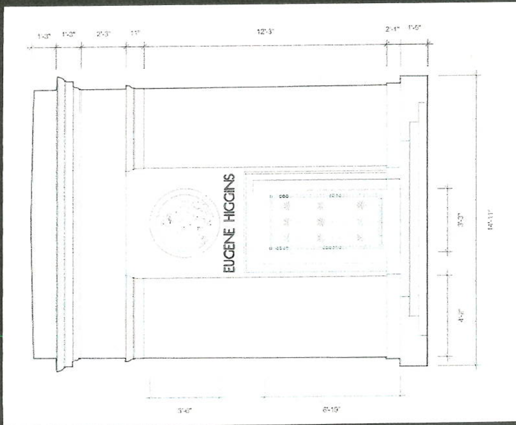
South elevation and plan.
