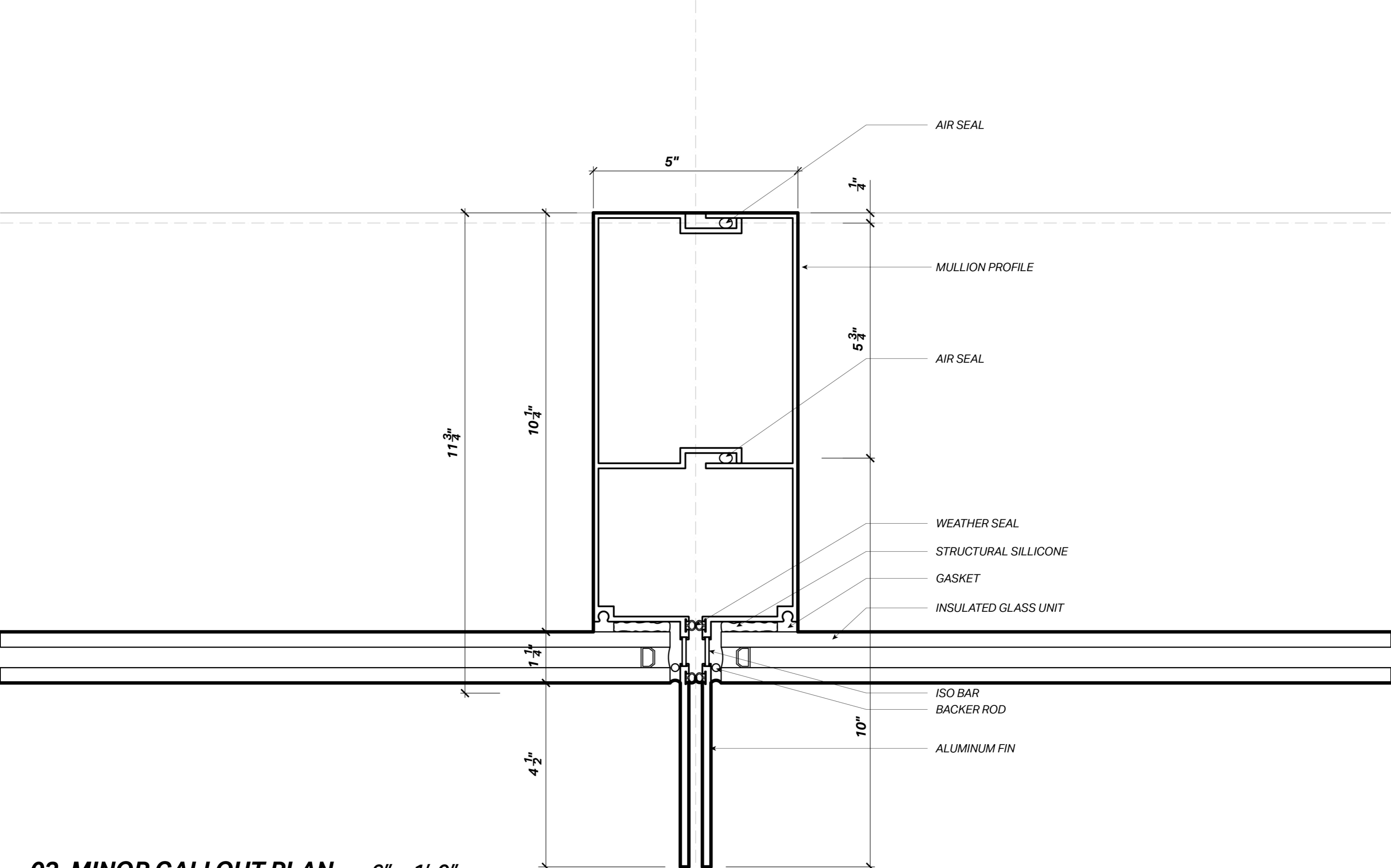
02_MINOR CALLOUT PLAN 6" = 1'-0"
