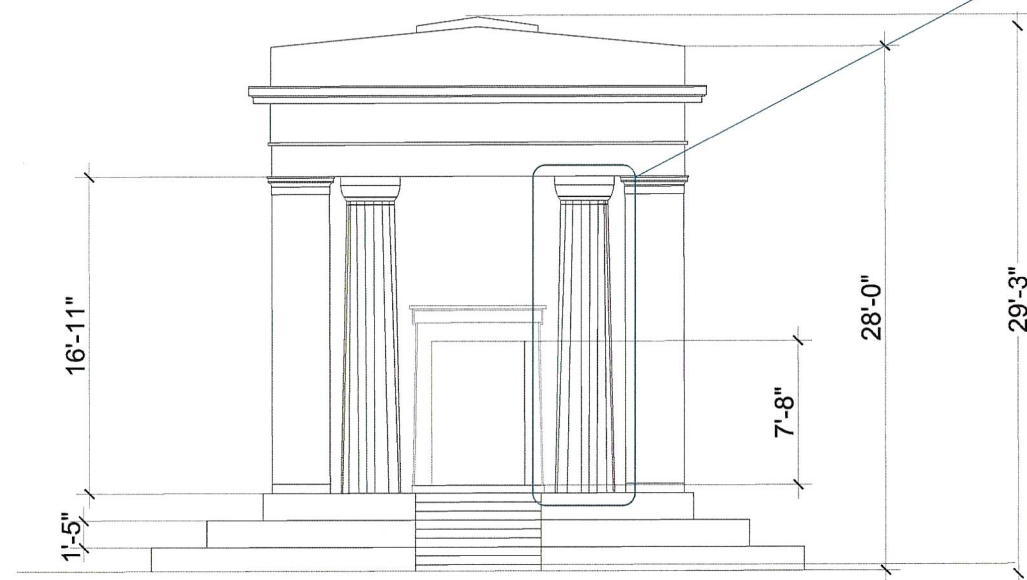
FRONT ELEVATION
