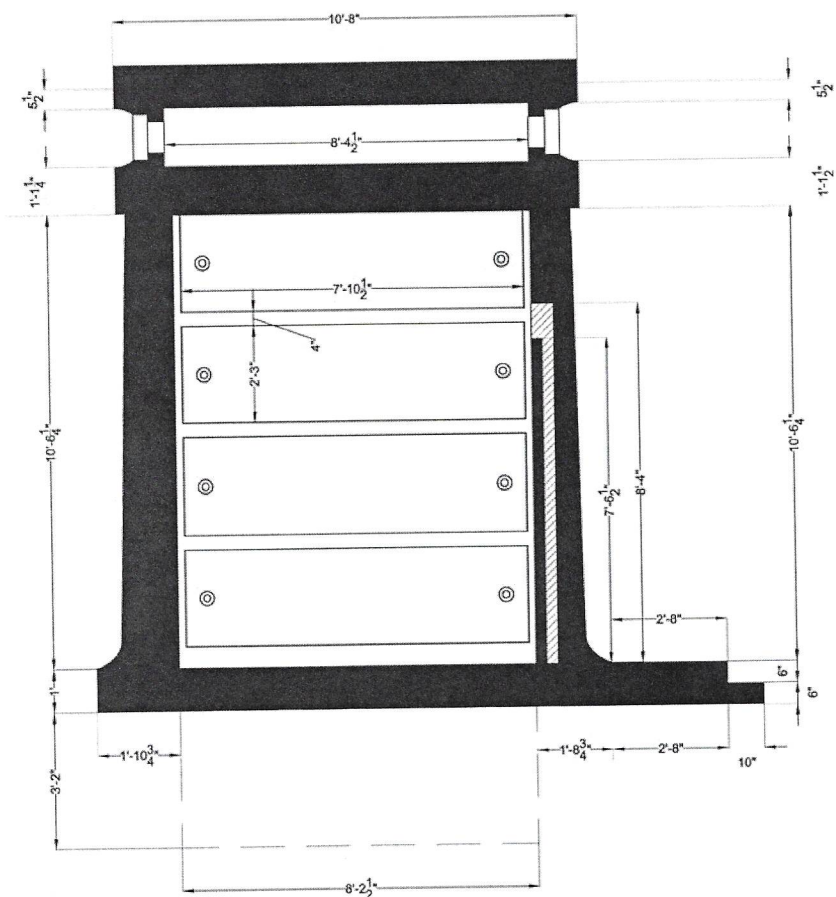
SECTION PLAN
